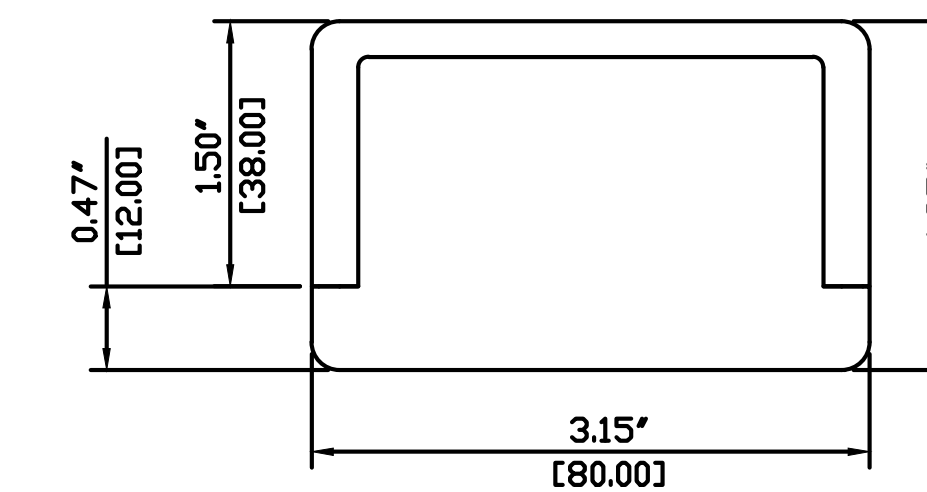
ASSEMBLY-END VIEW
