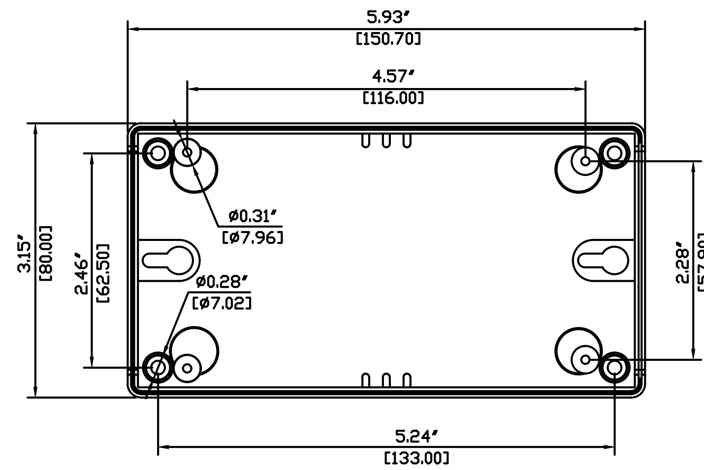
BOTTOM-INSIDE
