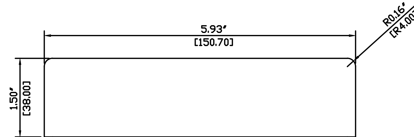
30066-TOP-SIDE VIEW
