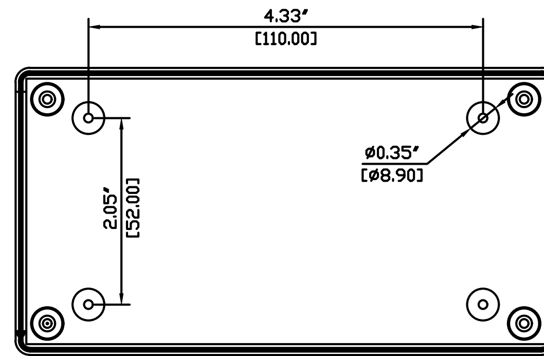
TOP-INSIDE
