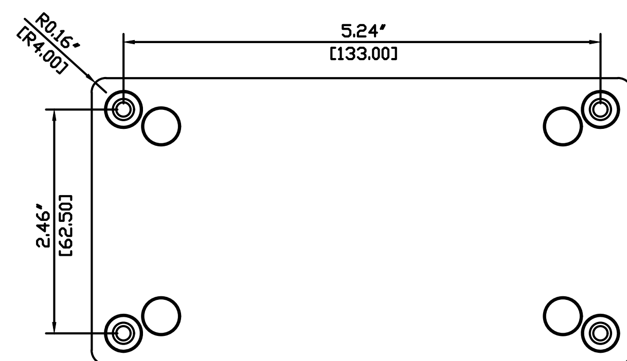
BOTTOM-OUTSIDE
