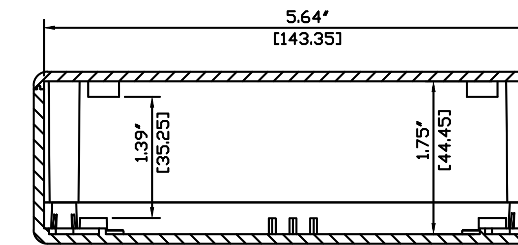
ASSEMBLY-SIDE SECTION
