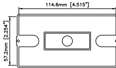
BOTTOM-OUTSIDE
