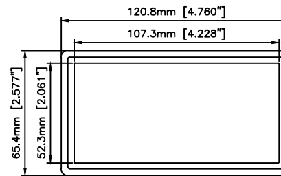
TOP-OUTSIDE
