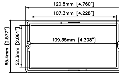
TOP-INSIDE
