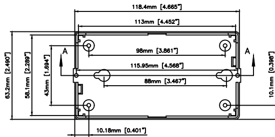
BOTTOM-INSIDE
