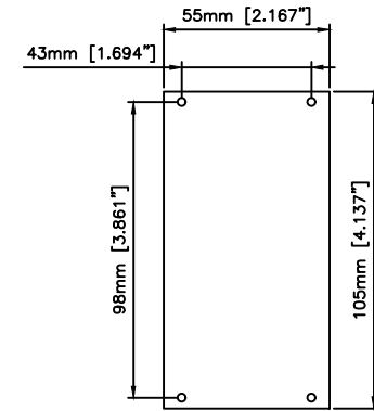
PCB
