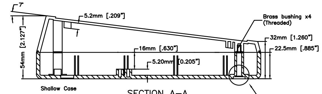
SECTION A-A 05-14-007/009 Shallow Bottom Version
