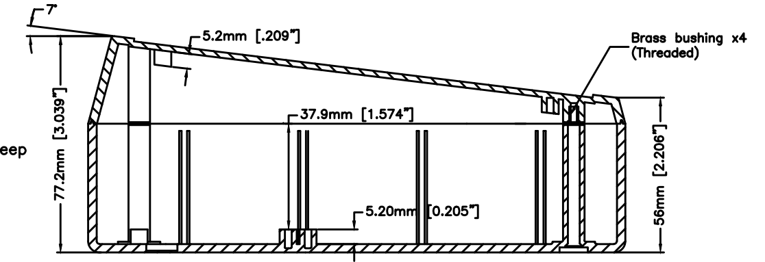
SECTION A-A 90-86-008 Deep Bottom Version
