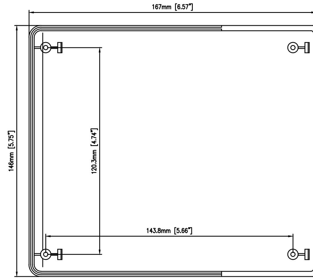
Top-Inside
