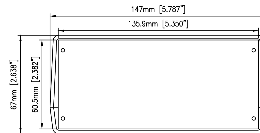
Front View
