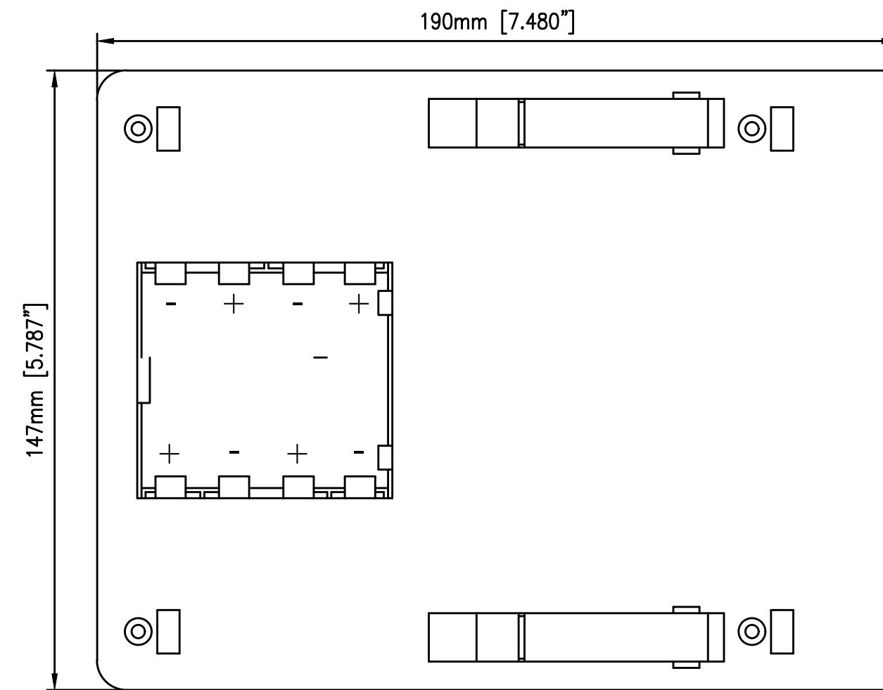
Bottom-Outside
