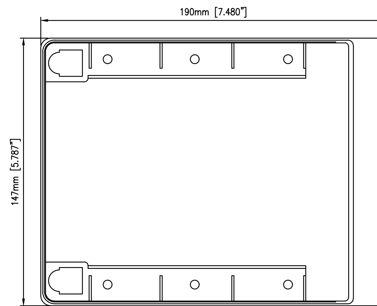
Insert-Top
