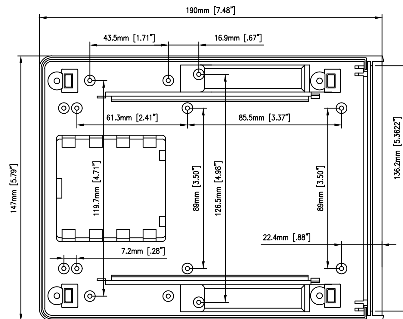
Bottom-Inside
