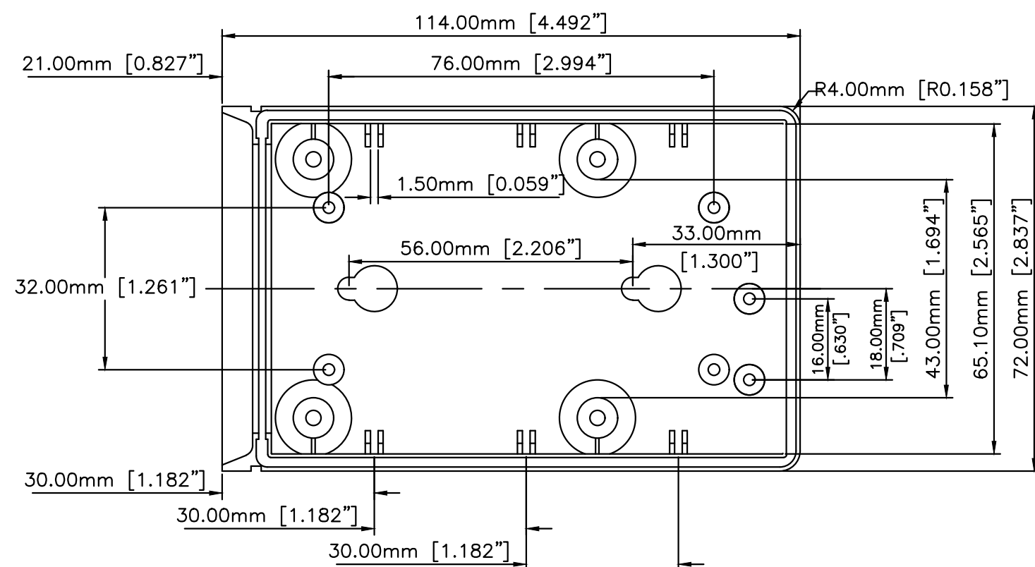
BOTTOM - INSIDE
