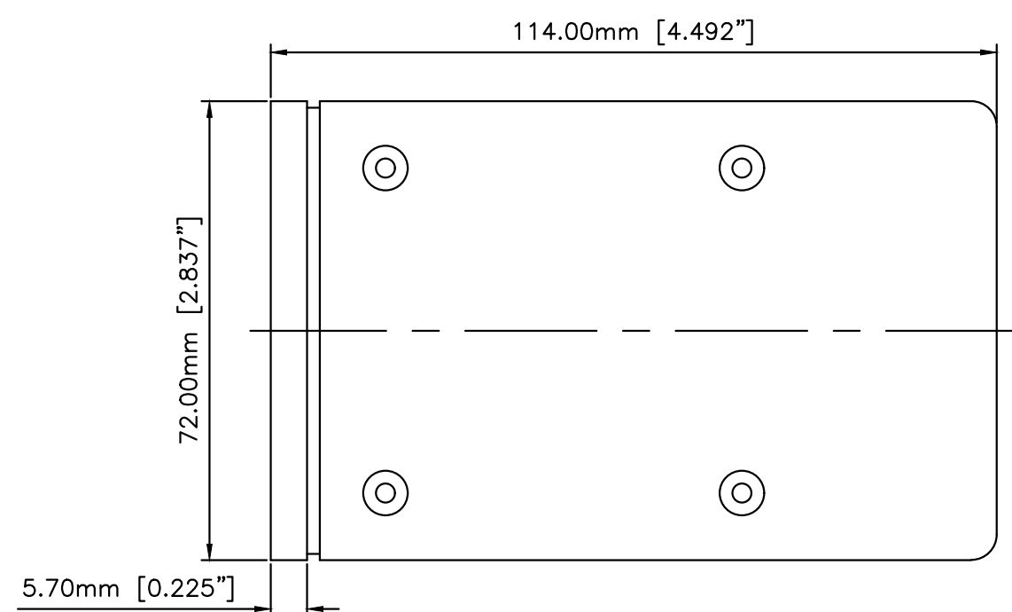
BOTTOM - OUTSIDE
