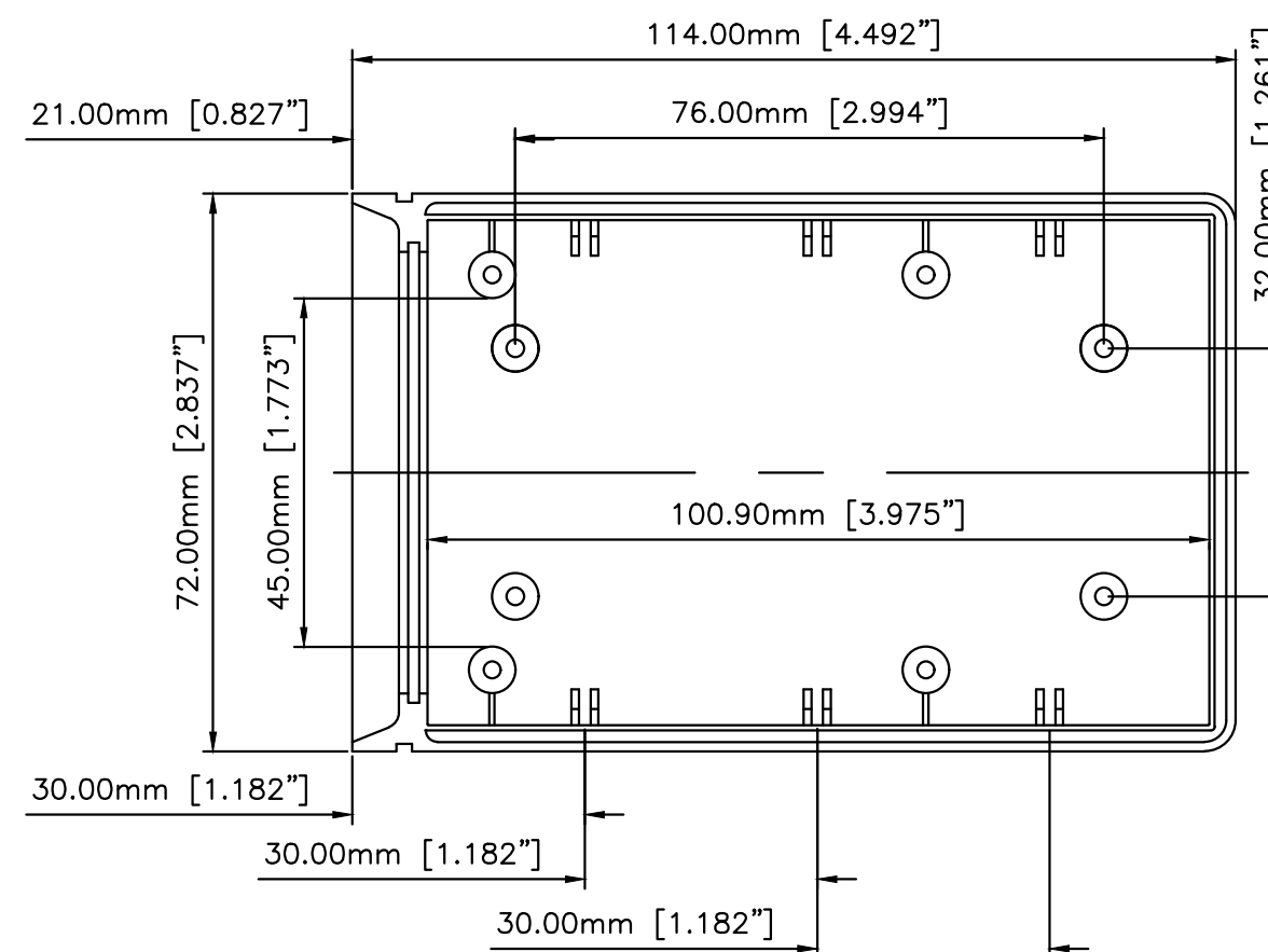
TOP - INSIDE
