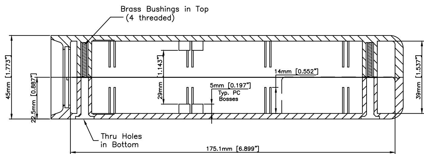
Side View
