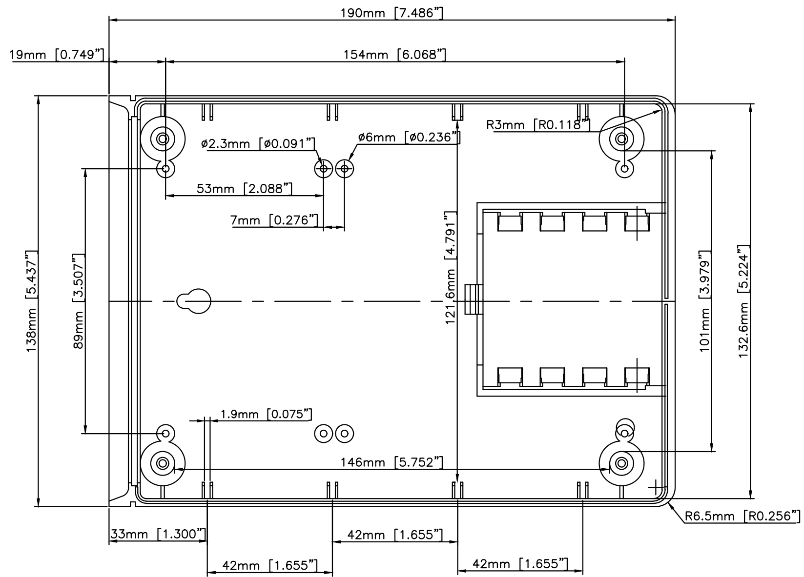
Bottom-Inside
