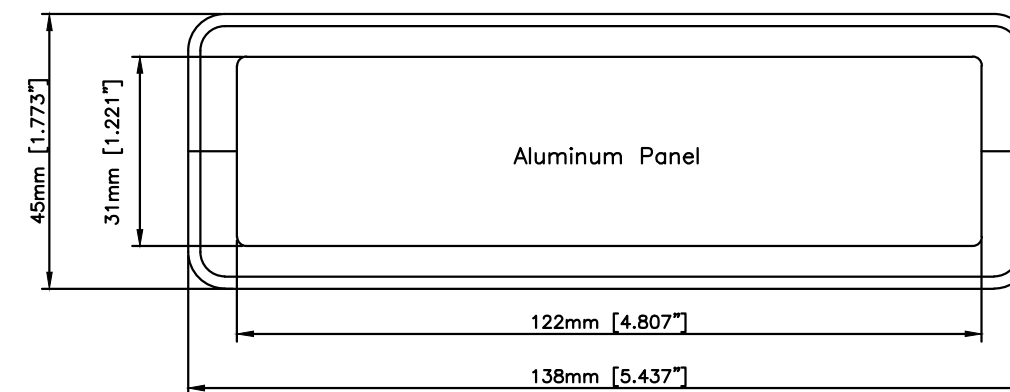
End View
