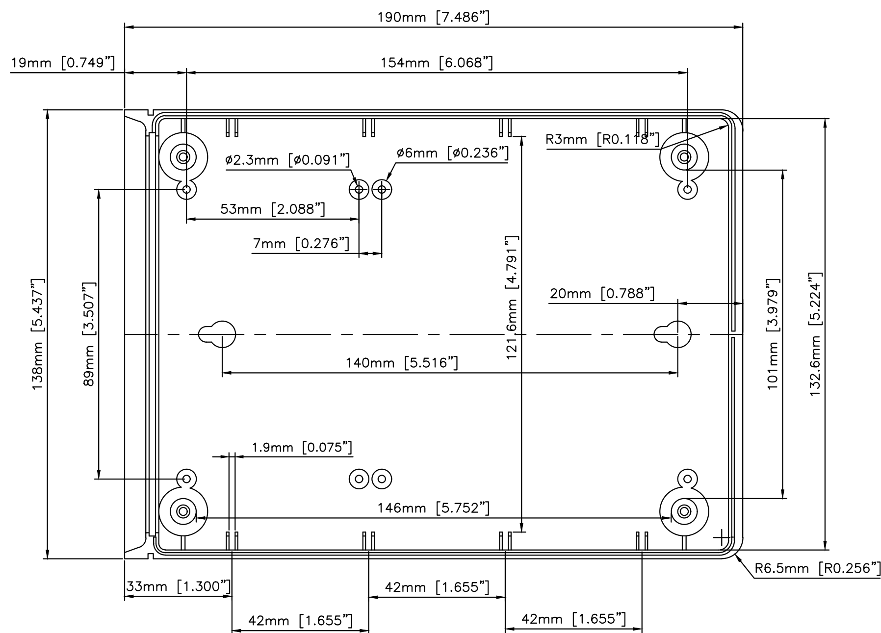
Bottom-Inside
