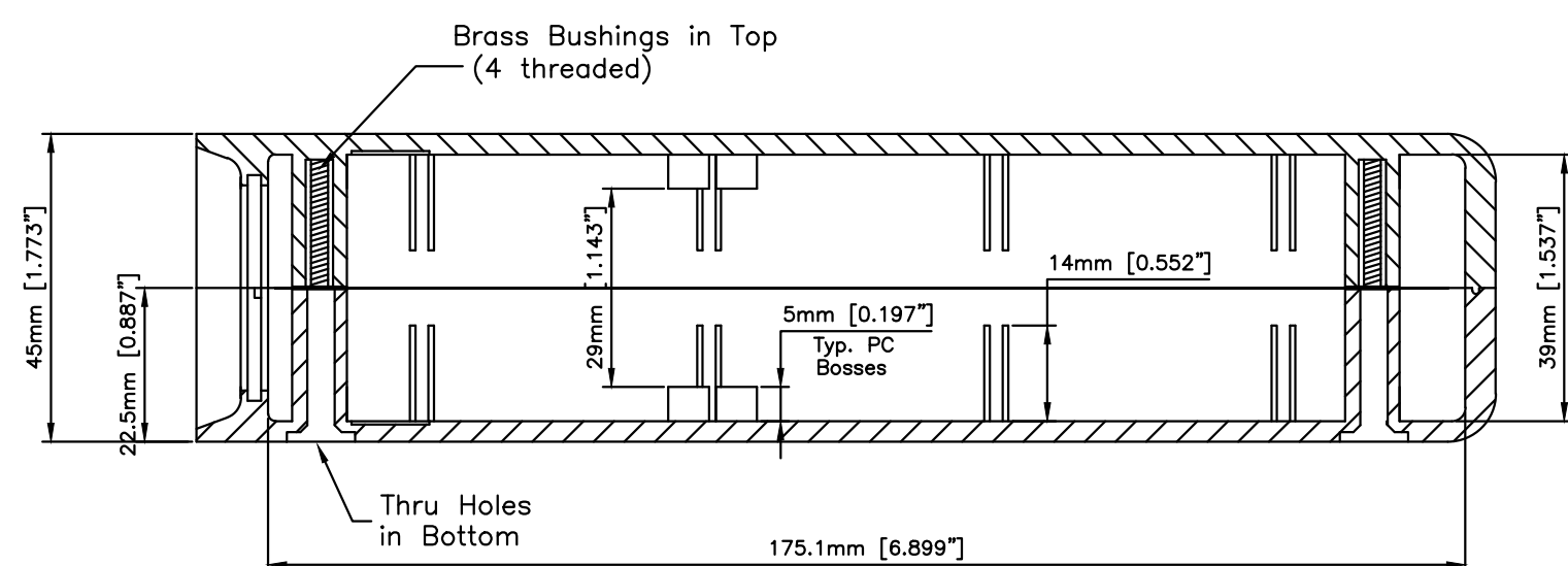
Side View
