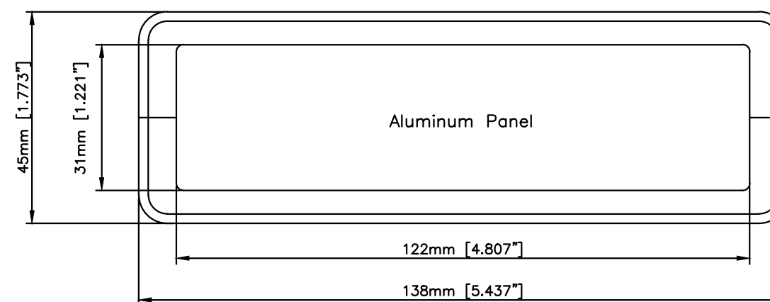
End View
