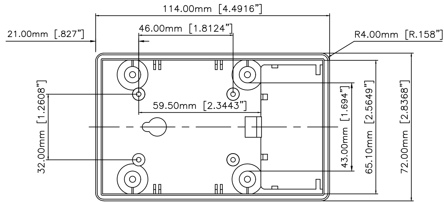
BOTTOM - INSIDE
