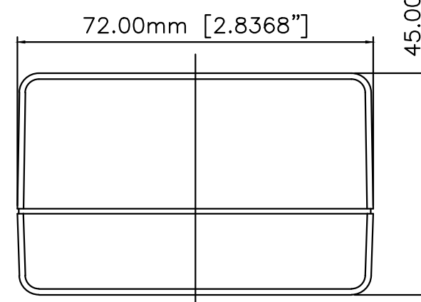
END VIEW
