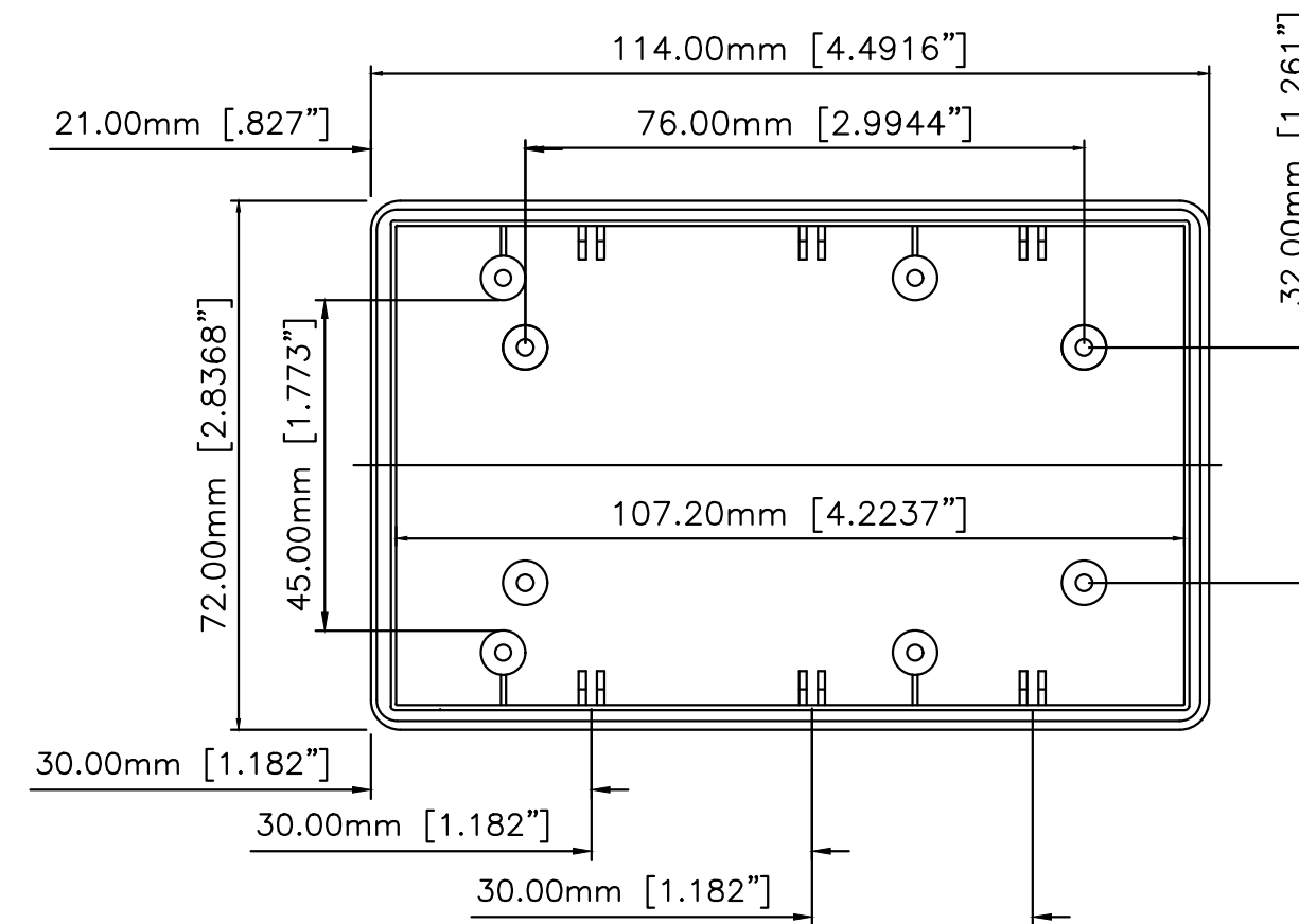
TOP - INSIDE
