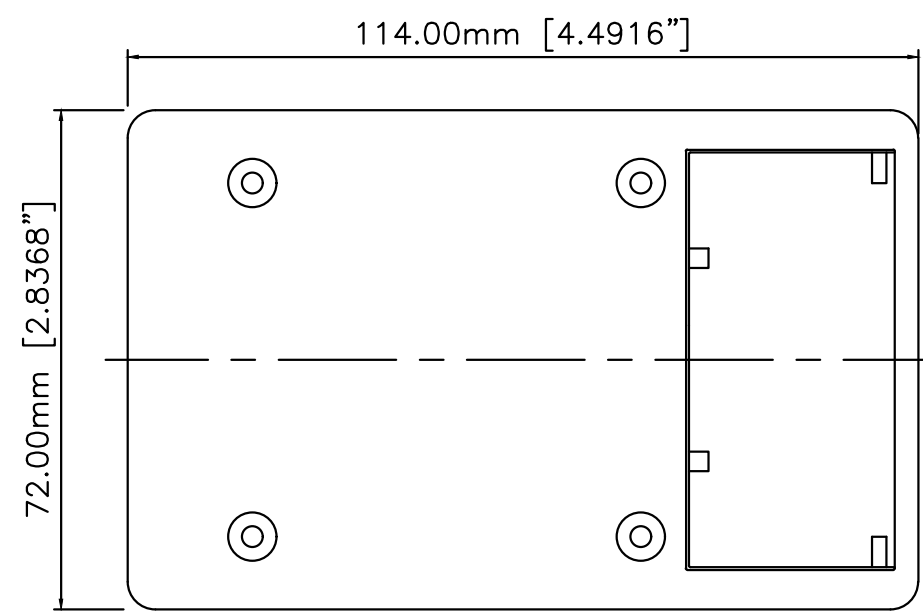
BOTTOM - OUTSIDE
