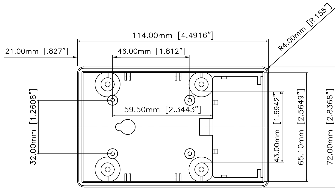
BOTTOM - INSIDE
