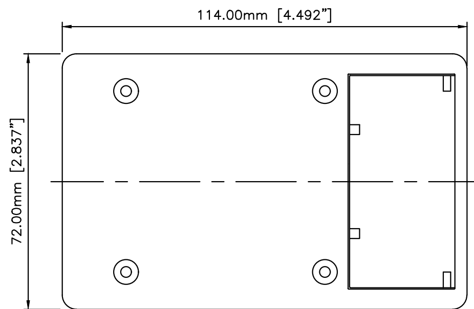
BOTTOM - OUTSIDE
