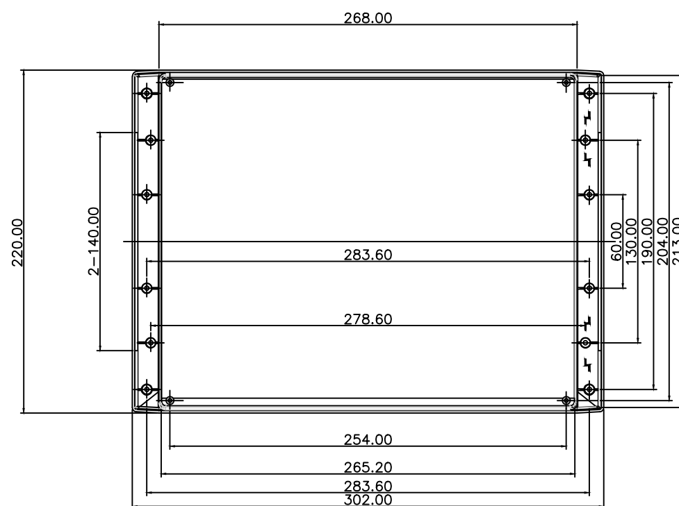
COVER INSIDE
