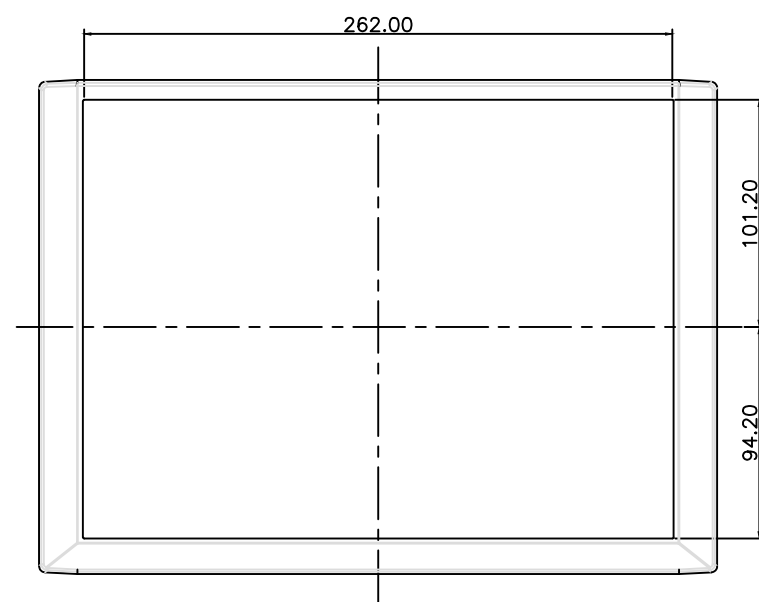
COVER OUTSIDE
