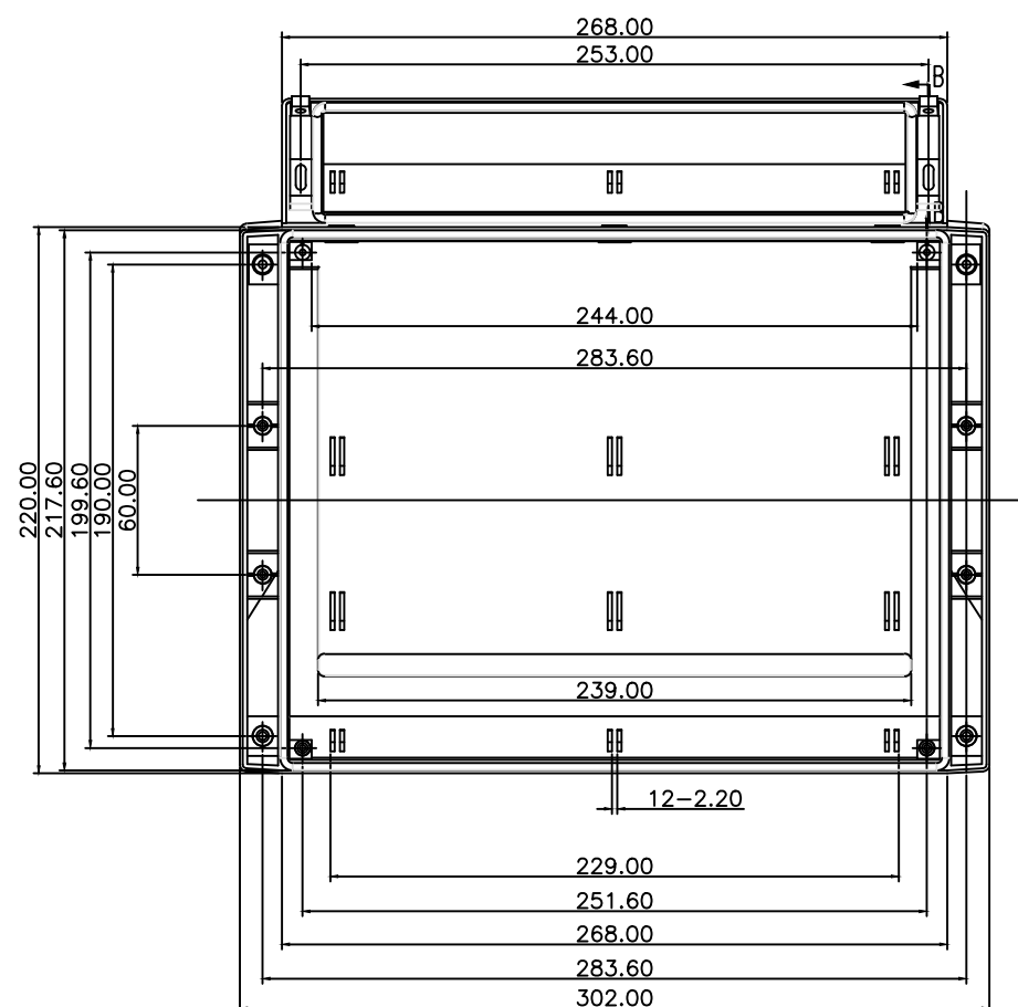
BOTTOM INSIDE
