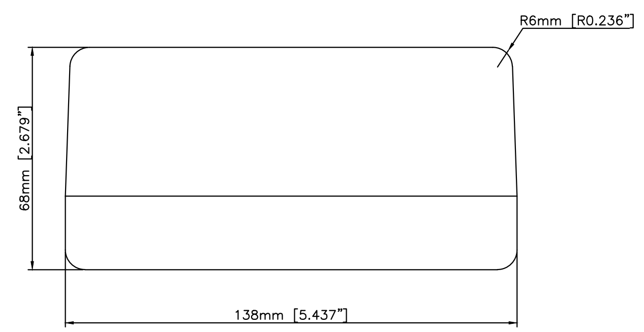
End View
