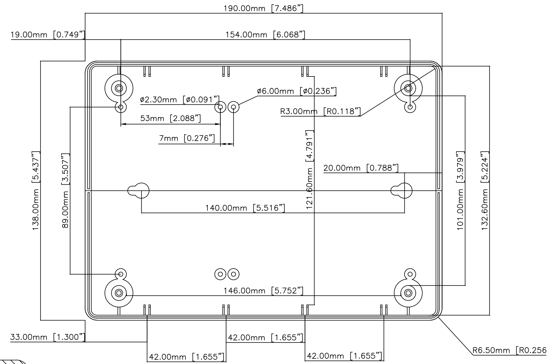
Top/Bottom - Inside
