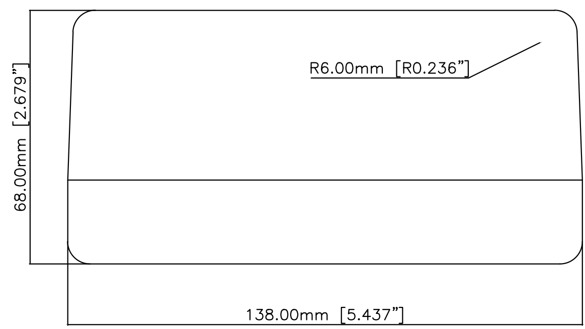
End View
